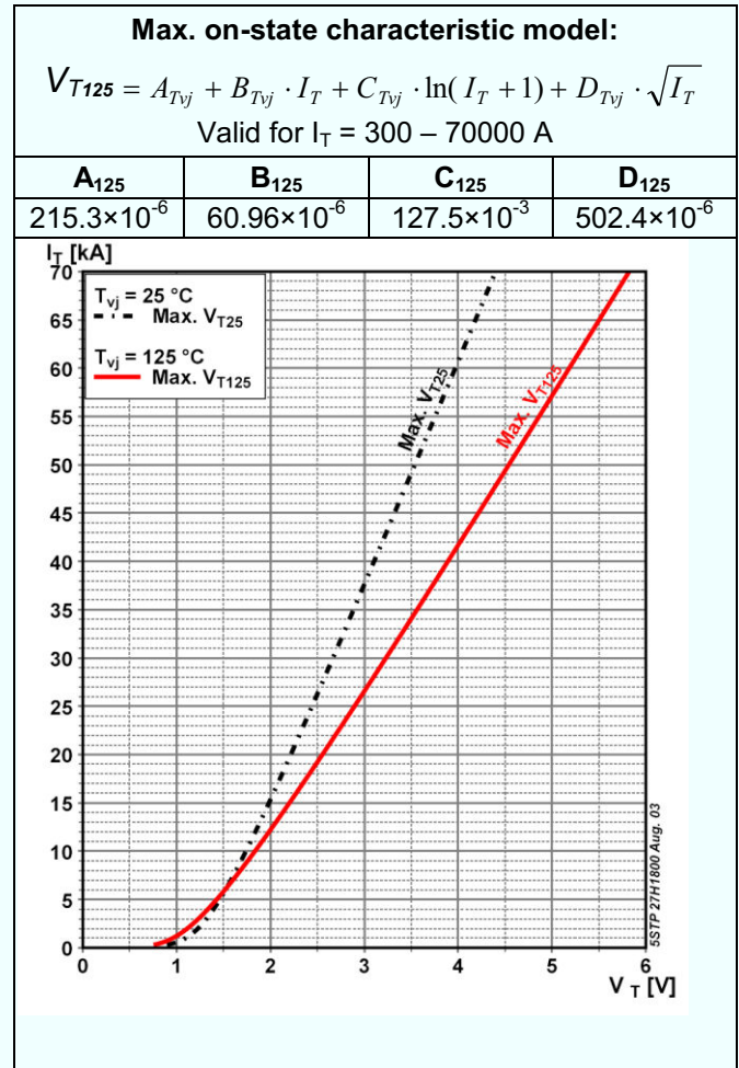
Fig. 3 On-state characteristics, T_j = 125^\circ\text{C} , 10ms half sine
